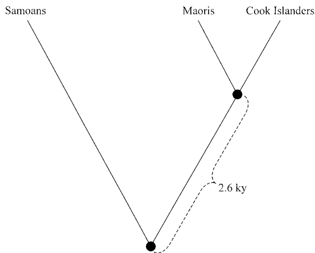
Figure 3 Genetic differentiation among the Polynesian populations. The time between the nodes was computed as \Delta T_D = (D'_1 - D_1)/2w (Zhivotovsky 2001), where D_1 is the average value of D_1 for population pairs (Samoans/Maoris and Samoans/Cook Islanders), and D'_1 is for the Maoris/Cook Islanders comparison.
